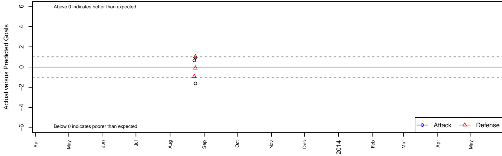
Juventus SC Earthquakes B01 Dots are actual minus expected GF (blue circles) and GA (red triangles). Blue line is smoothed change in attack strength. Red is smoothed change in defense strength.
